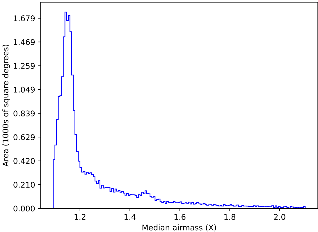
telescope_jerk_v3.5_10yrs All sky all bands: Median airmass
