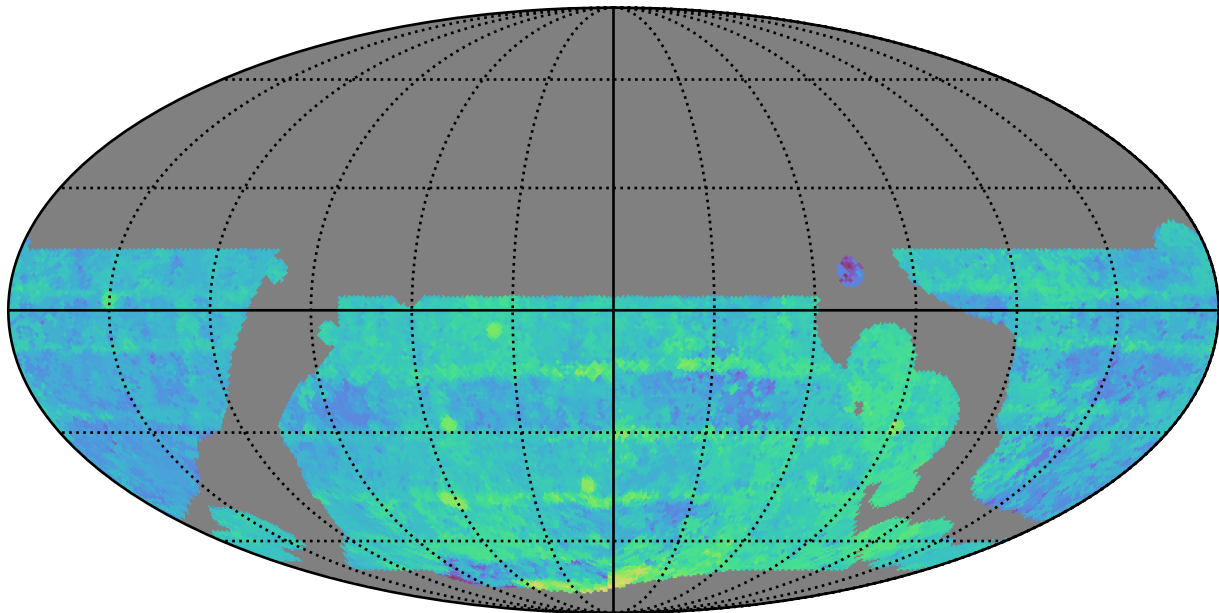
telescope_jerk_v3.5_10yrs WFD z band: Median Season Length
