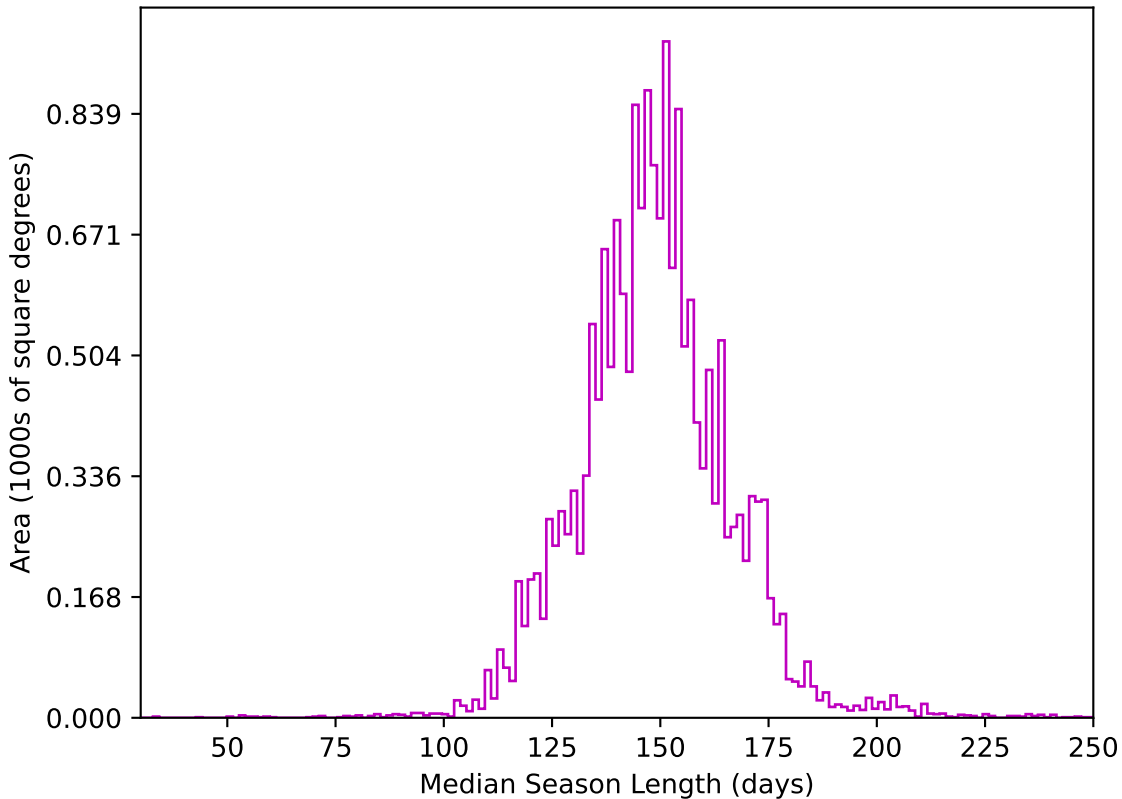
telescope_jerk_v3.5_10yrs WFD z band: Median Season Length
