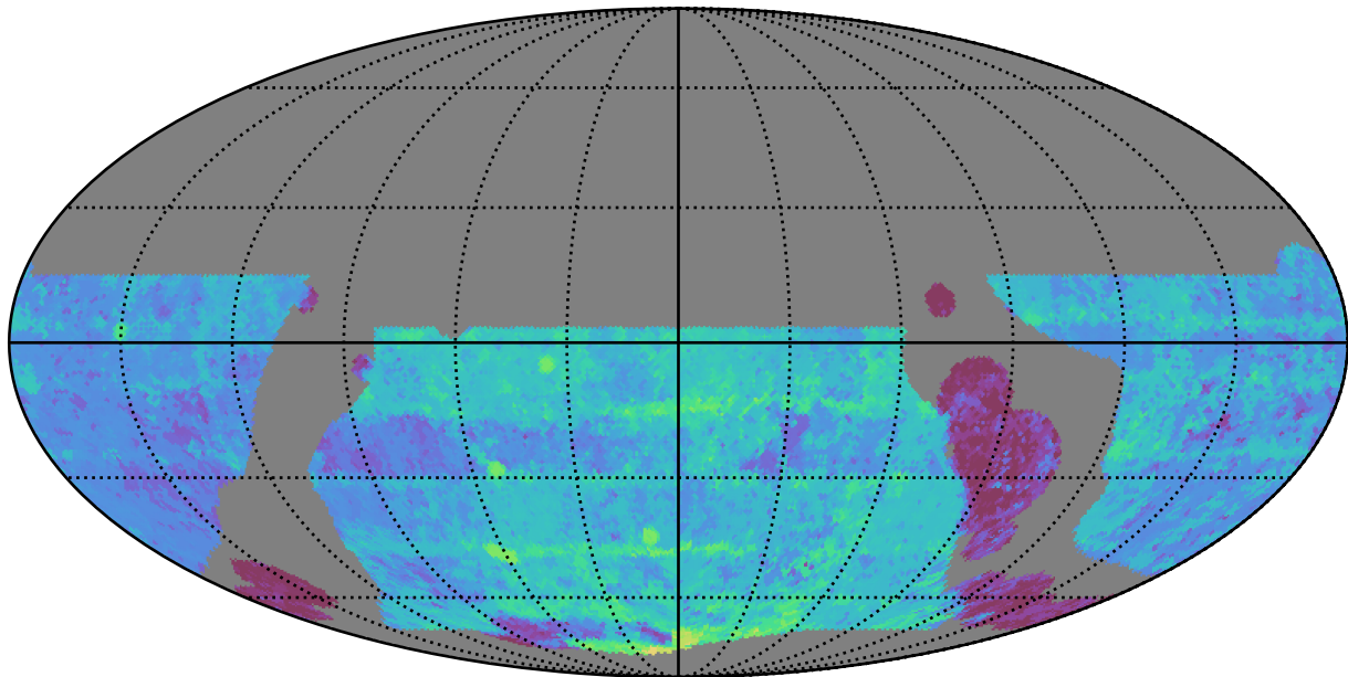
telescope_jerk_v3.5_10yrs WFD y band: Median Season Length
