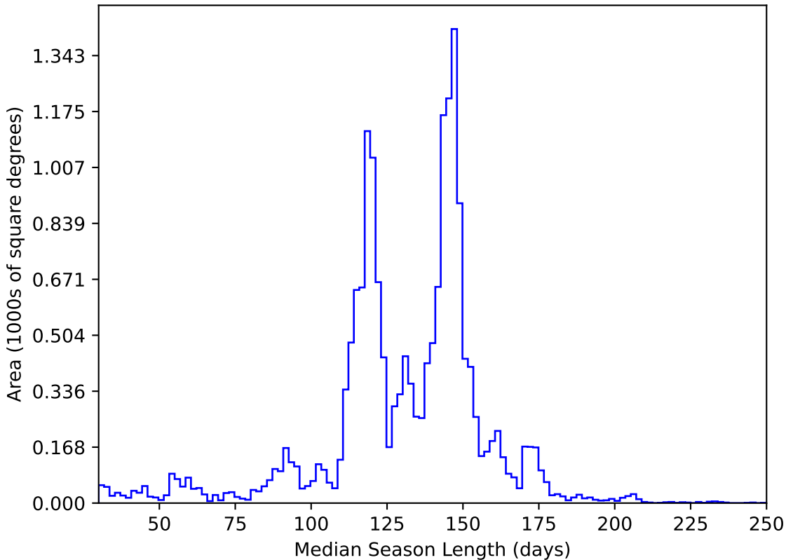
telescope_jerk_v3.5_10yrs WFD y band: Median Season Length
