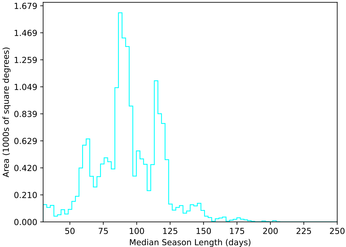
telescope_jerk_v3.5_10yrs WFD u band: Median Season Length
