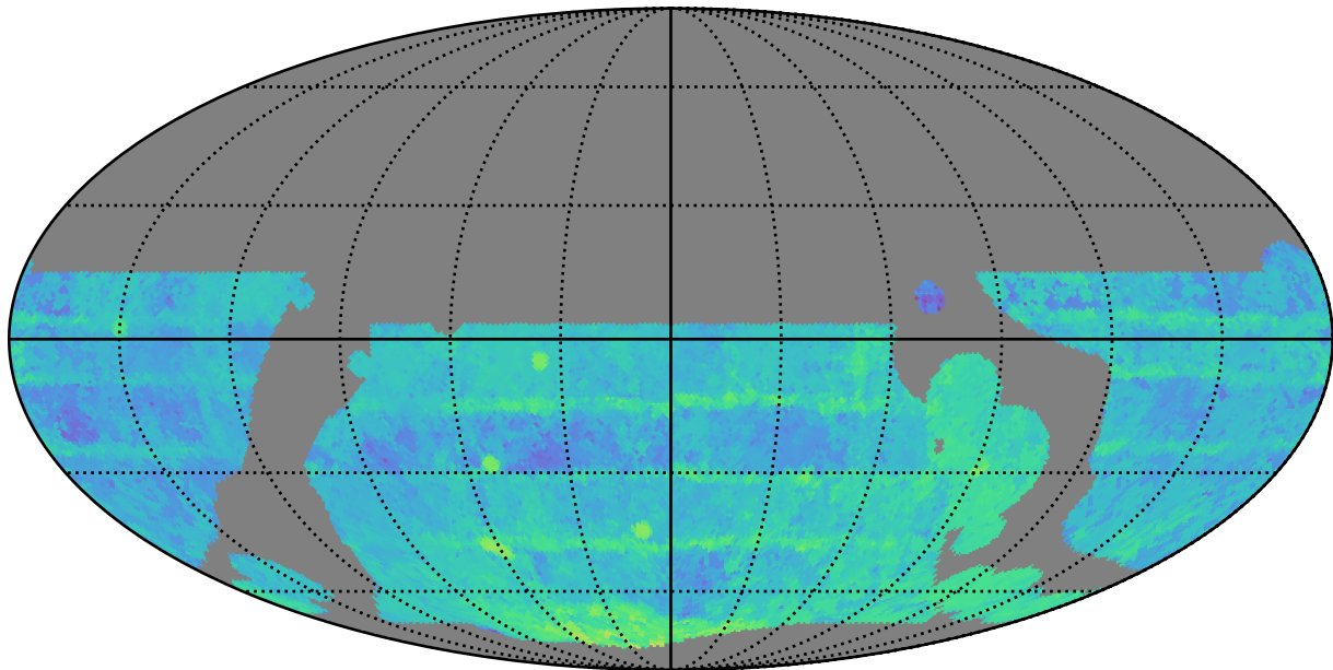
telescope_jerk_v3.5_10yrs WFD r band: Median Season Length
