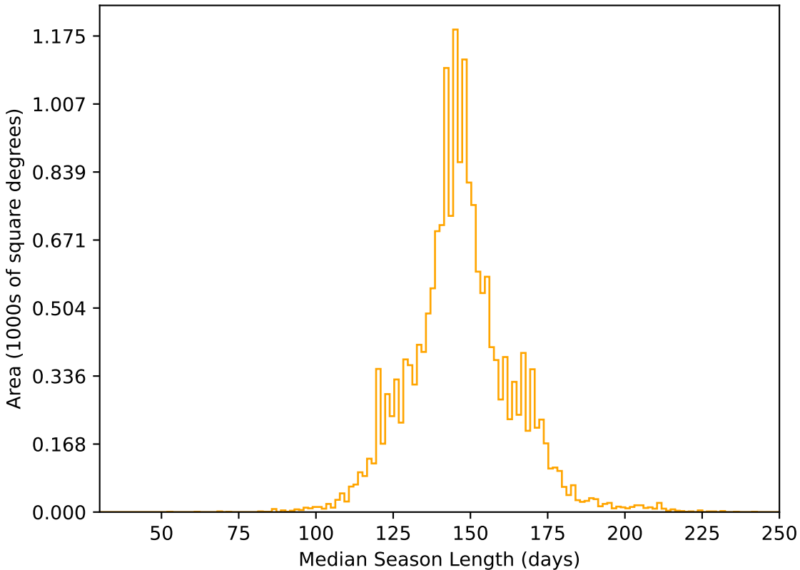
telescope_jerk_v3.5_10yrs WFD r band: Median Season Length
