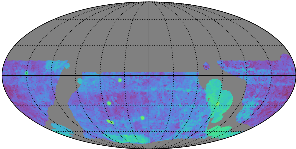
telescope_jerk_v3.5_10yrs WFD g band: Median Season Length
