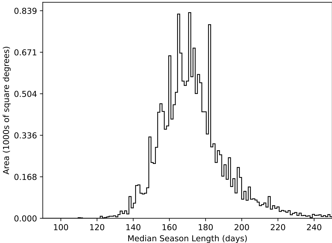
telescope_jerk_v3.5_10yrs WFD all bands: Median Season Length
