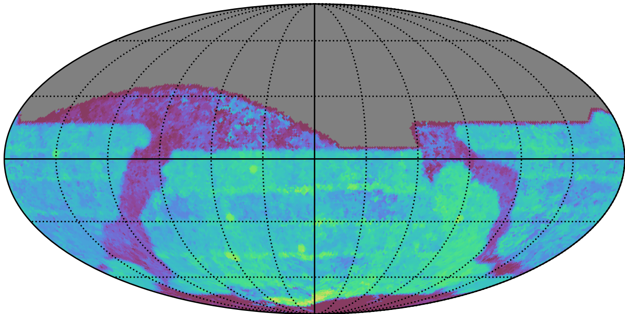
telescope_jerk_v3.5_10yrs All sky z band: Median Season Length
