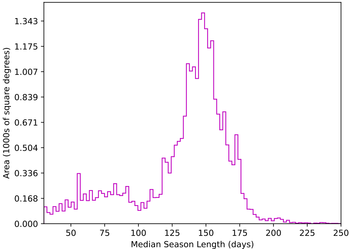
telescope_jerk_v3.5_10yrs All sky z band: Median Season Length
