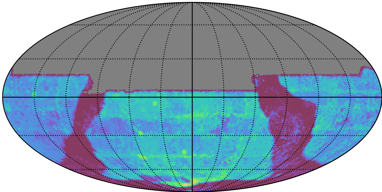
telescope_jerk_v3.5_10yrs All sky y band: Median Season Length
