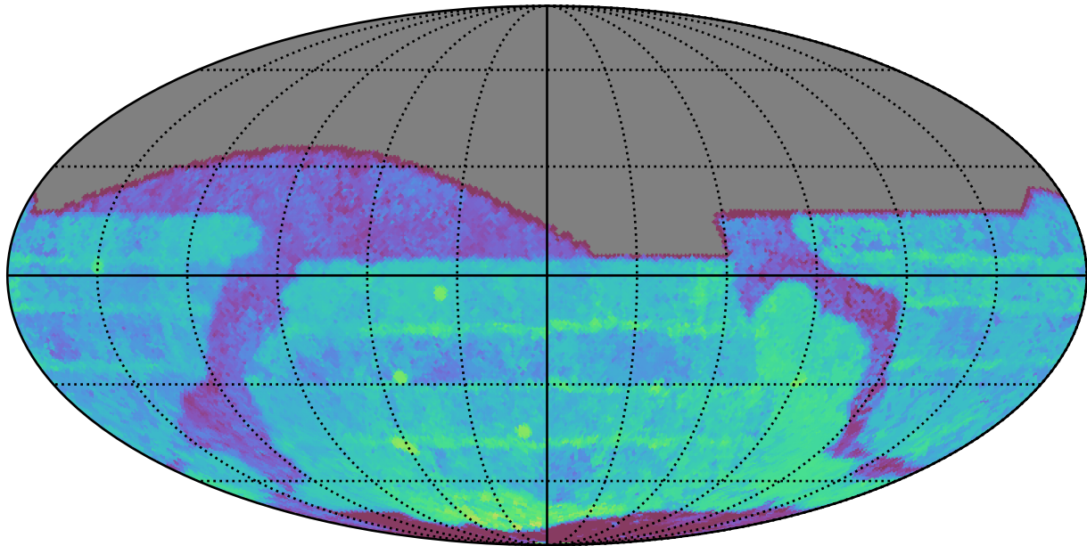
telescope_jerk_v3.5_10yrs All sky r band: Median Season Length
