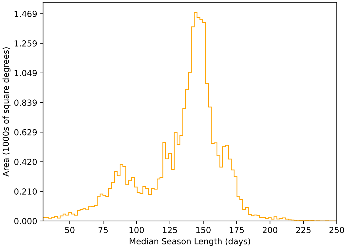
telescope_jerk_v3.5_10yrs All sky r band: Median Season Length
