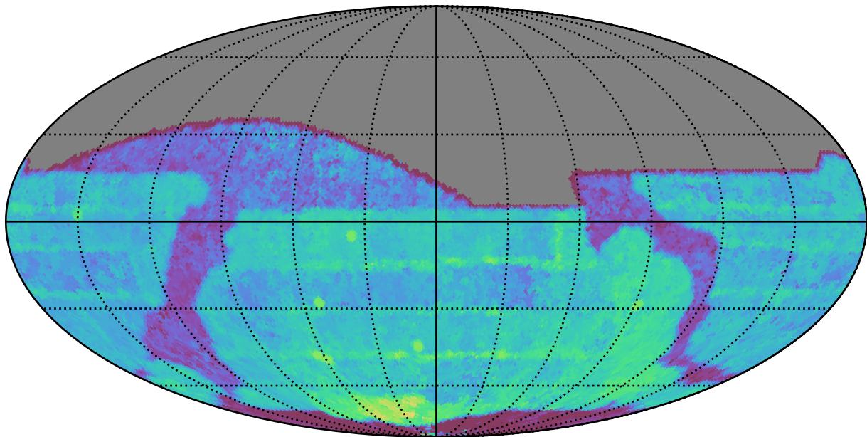
telescope_jerk_v3.5_10yrs All sky i band: Median Season Length
