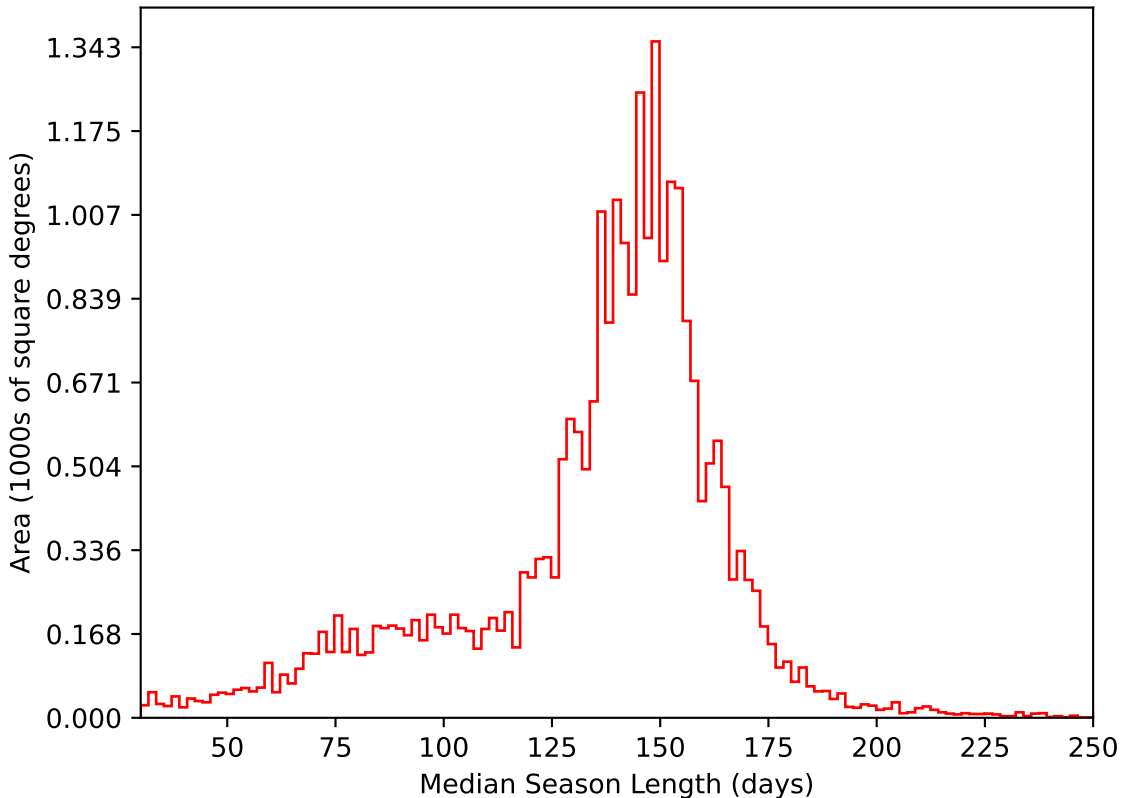
telescope_jerk_v3.5_10yrs All sky i band: Median Season Length
