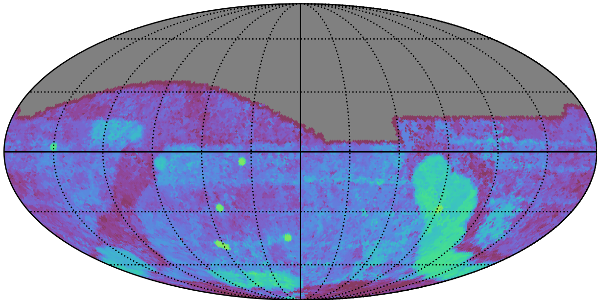
telescope_jerk_v3.5_10yrs All sky g band: Median Season Length
