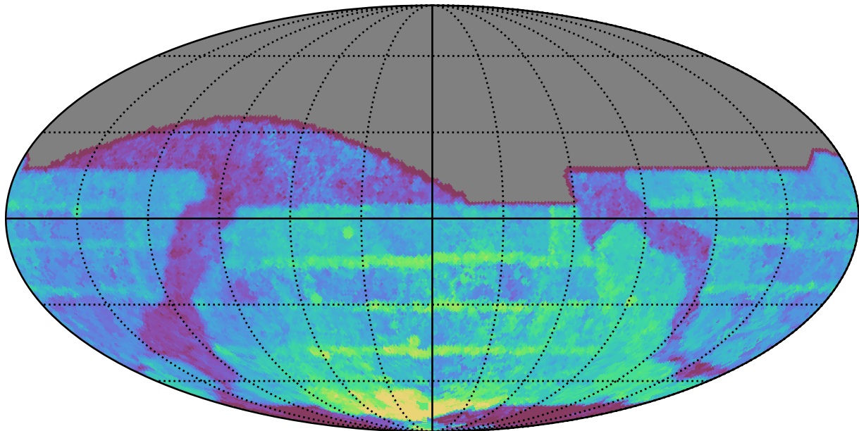
telescope_jerk_v3.5_10yrs All sky all bands: Median Season Length
