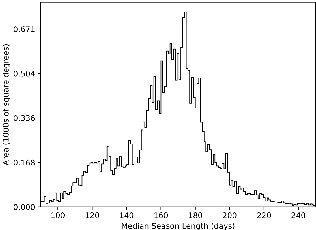
telescope_jerk_v3.5_10yrs All sky all bands: Median Season Length
