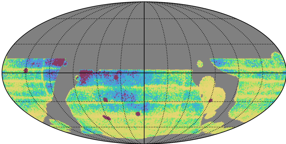
telescope_jerk_v3.5_10yrs WFD: Median Intra-Night Gap
