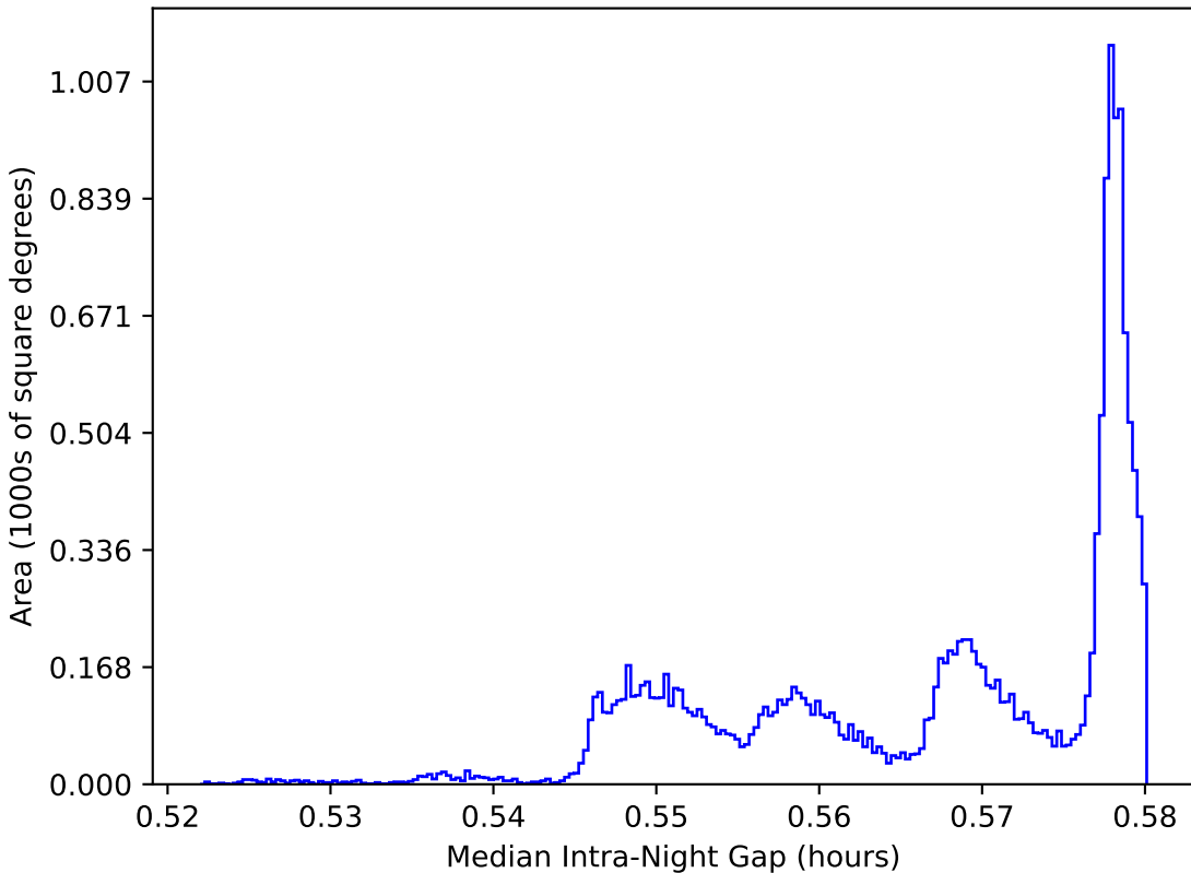
telescope_jerk_v3.5_10yrs WFD: Median Intra-Night Gap
