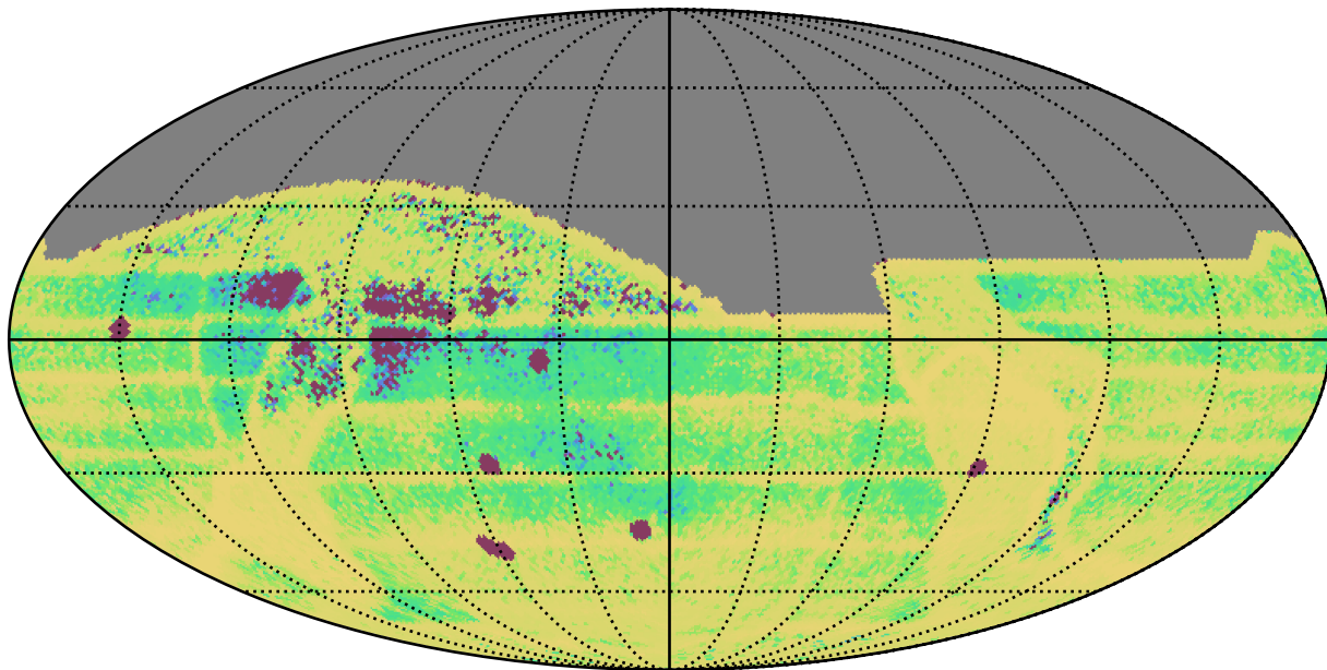
telescope_jerk_v3.5_10yrs All sky: Median Intra-Night Gap
