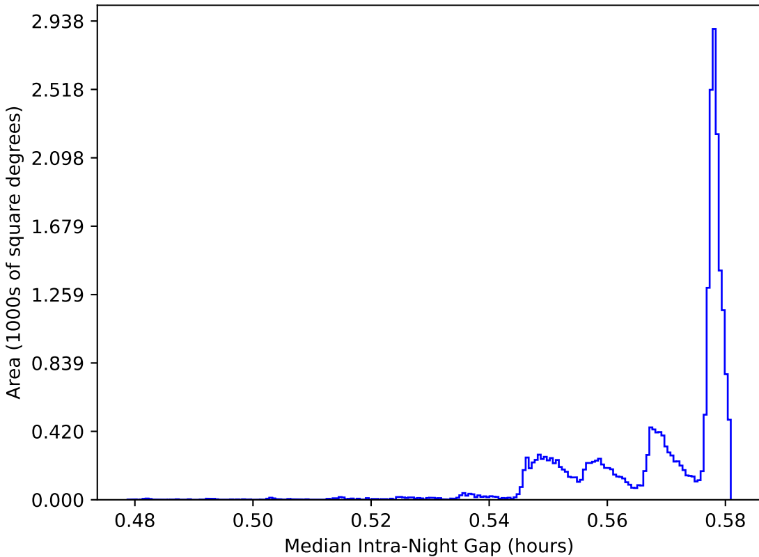
telescope_jerk_v3.5_10yrs All sky: Median Intra-Night Gap
