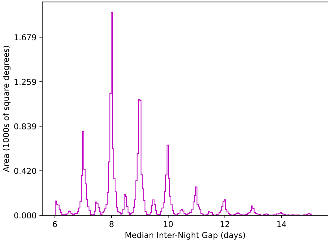
telescope_jerk_v3.5_10yrs WFD z band: Median Inter-Night Gap
