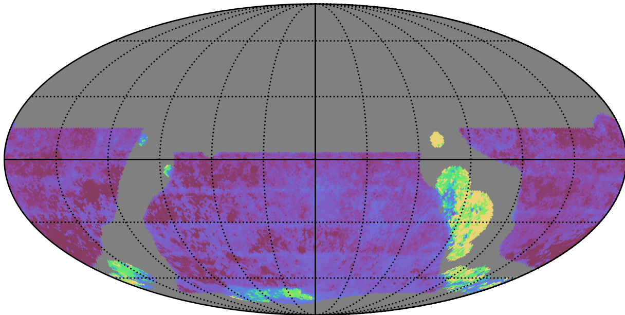
telescope_jerk_v3.5_10yrs WFD y band: Median Inter-Night Gap
