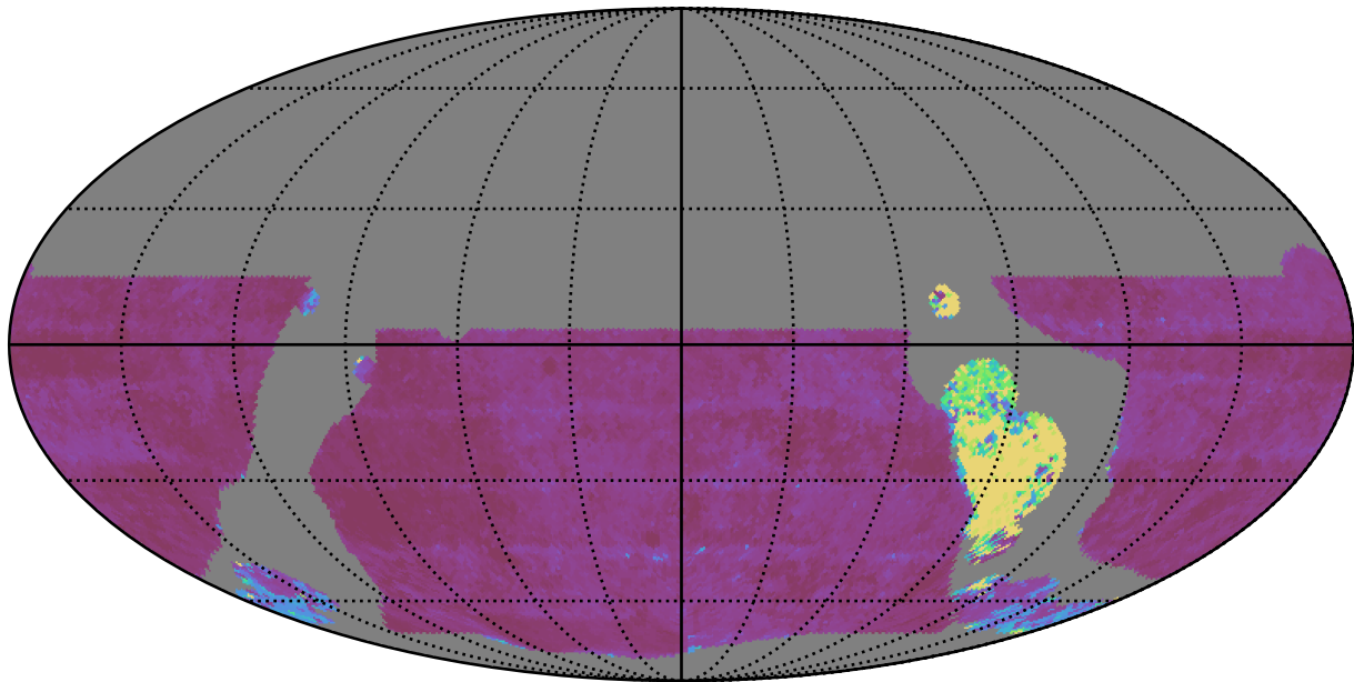
telescope_jerk_v3.5_10yrs WFD u band: Median Inter-Night Gap
