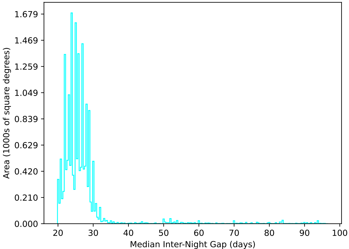
telescope_jerk_v3.5_10yrs WFD u band: Median Inter-Night Gap
