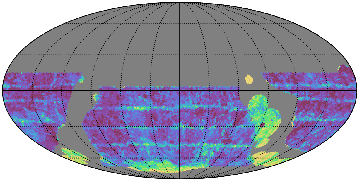
telescope_jerk_v3.5_10yrs WFD r band: Median Inter-Night Gap
