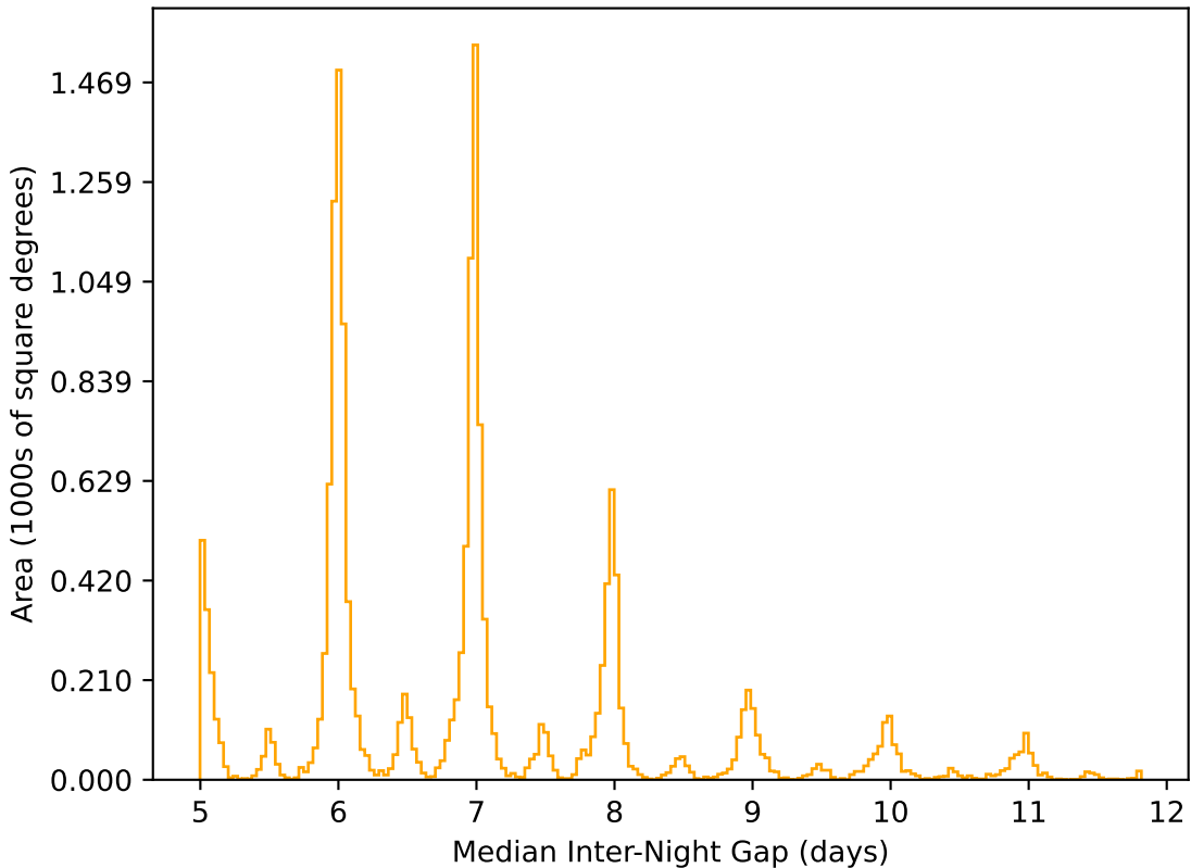
telescope_jerk_v3.5_10yrs WFD r band: Median Inter-Night Gap
