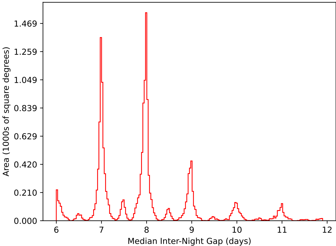
telescope_jerk_v3.5_10yrs WFD i band: Median Inter-Night Gap
