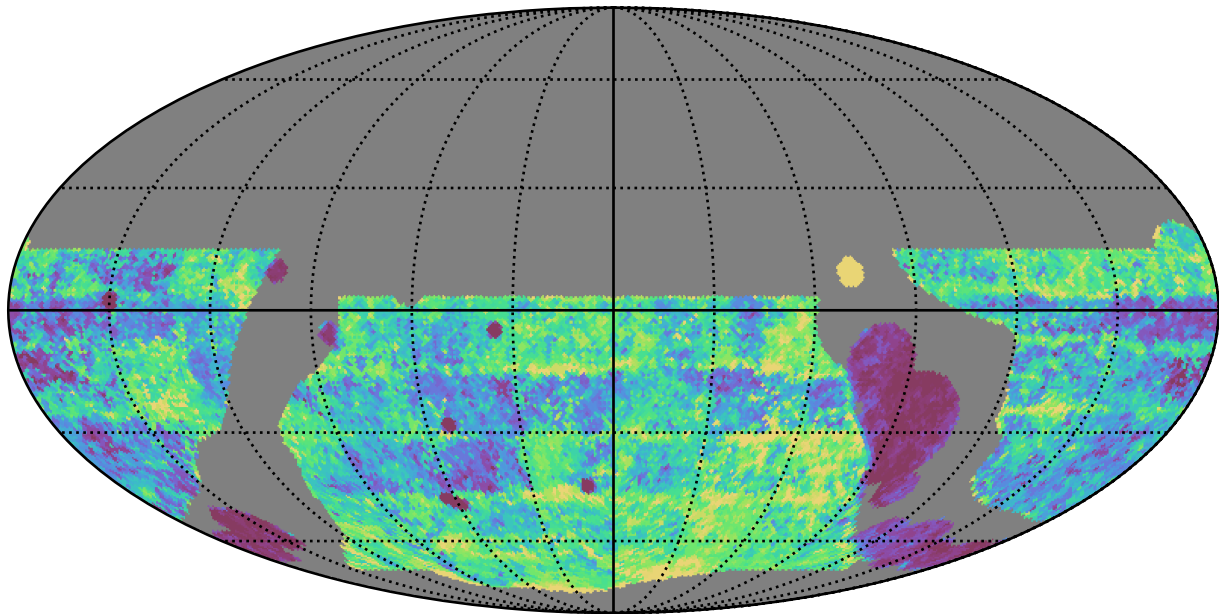
telescope_jerk_v3.5_10yrs WFD g band: Median Inter-Night Gap
