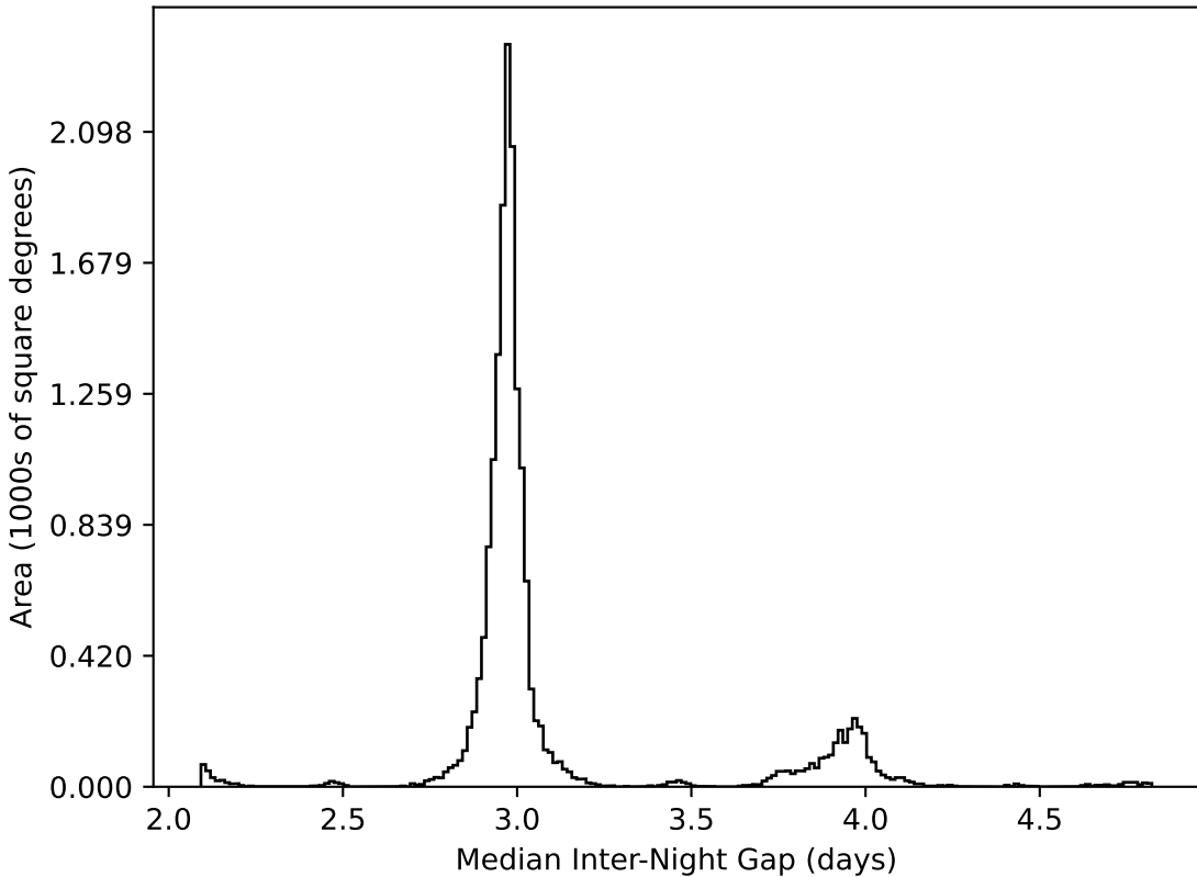
telescope_jerk_v3.5_10yrs WFD all bands: Median Inter-Night Gap
