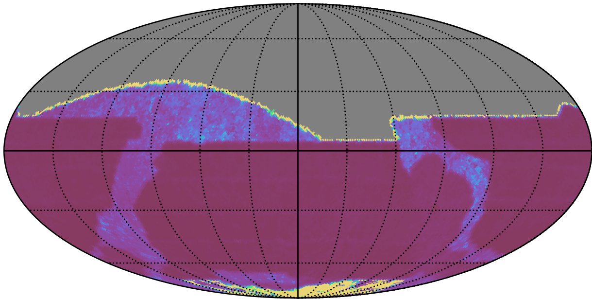
telescope_jerk_v3.5_10yrs All sky z band: Median Inter-Night Gap
