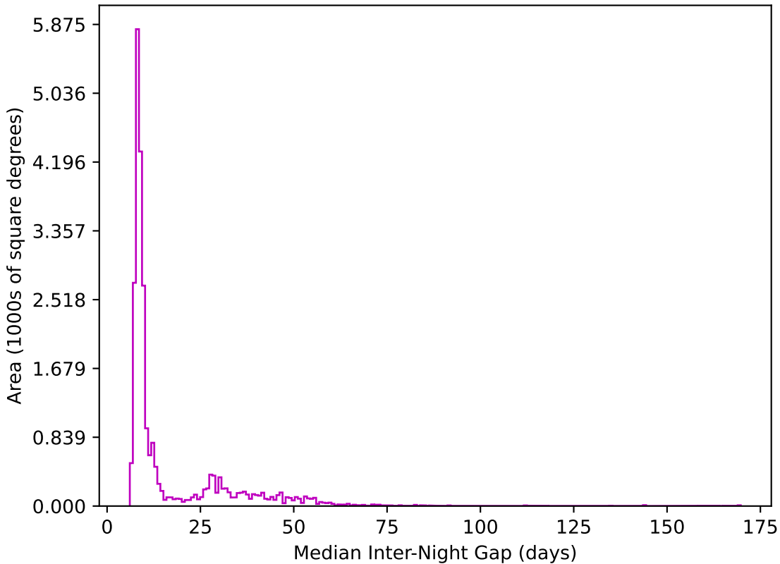
telescope_jerk_v3.5_10yrs All sky z band: Median Inter-Night Gap
