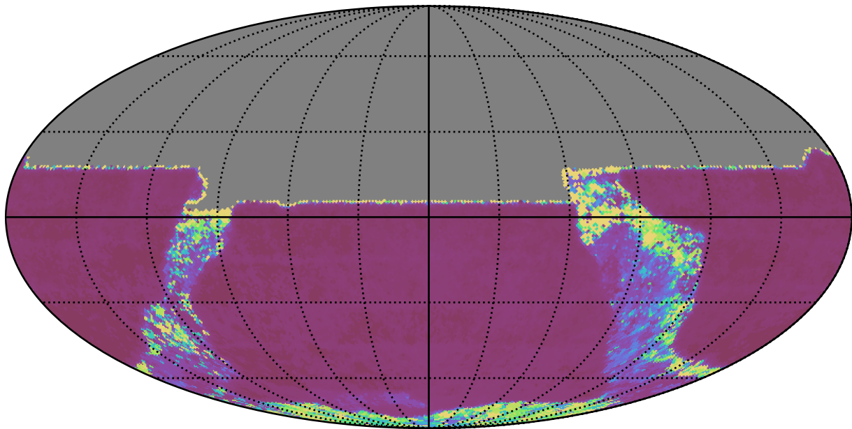
telescope_jerk_v3.5_10yrs All sky y band: Median Inter-Night Gap
