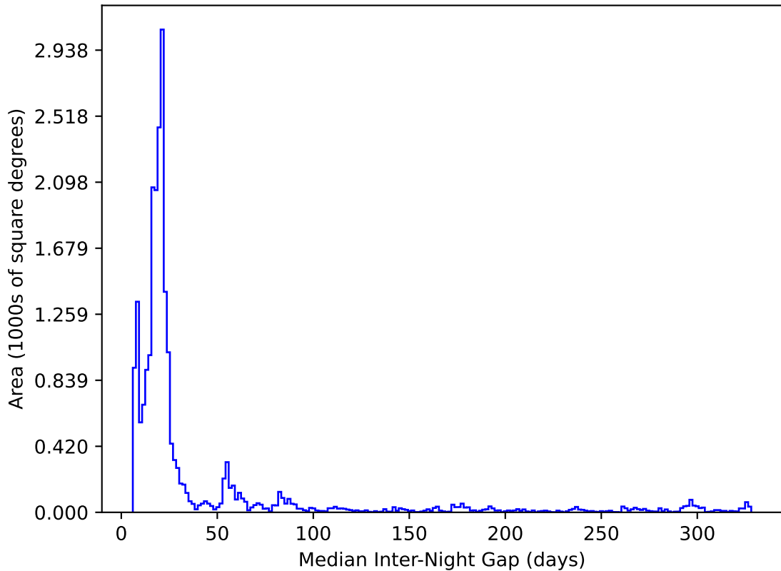
telescope_jerk_v3.5_10yrs All sky y band: Median Inter-Night Gap
