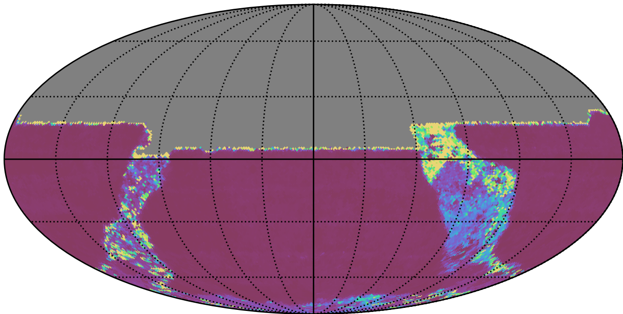
telescope_jerk_v3.5_10yrs All sky u band: Median Inter-Night Gap
