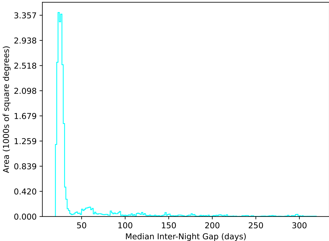
telescope_jerk_v3.5_10yrs All sky u band: Median Inter-Night Gap
