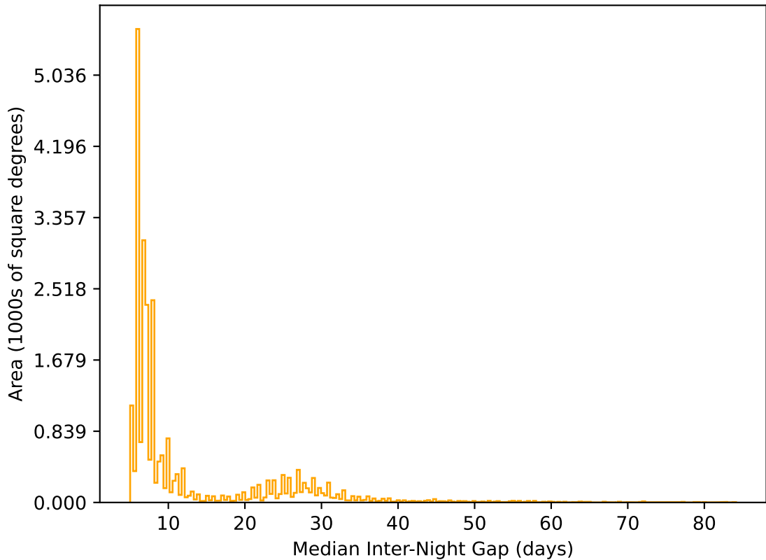
telescope_jerk_v3.5_10yrs All sky r band: Median Inter-Night Gap
