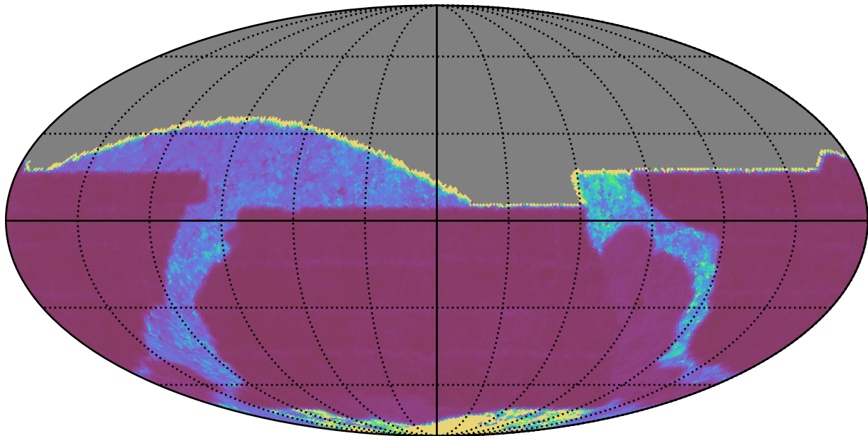
telescope_jerk_v3.5_10yrs All sky i band: Median Inter-Night Gap
