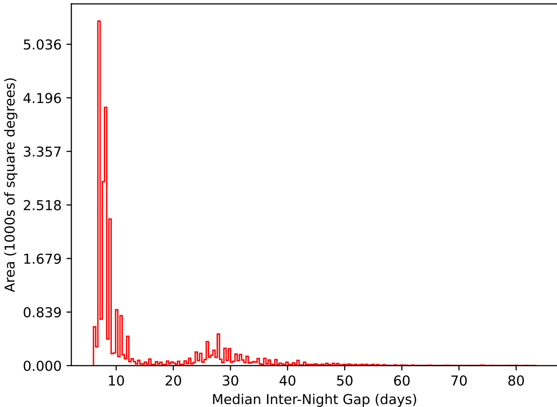
telescope_jerk_v3.5_10yrs All sky i band: Median Inter-Night Gap
