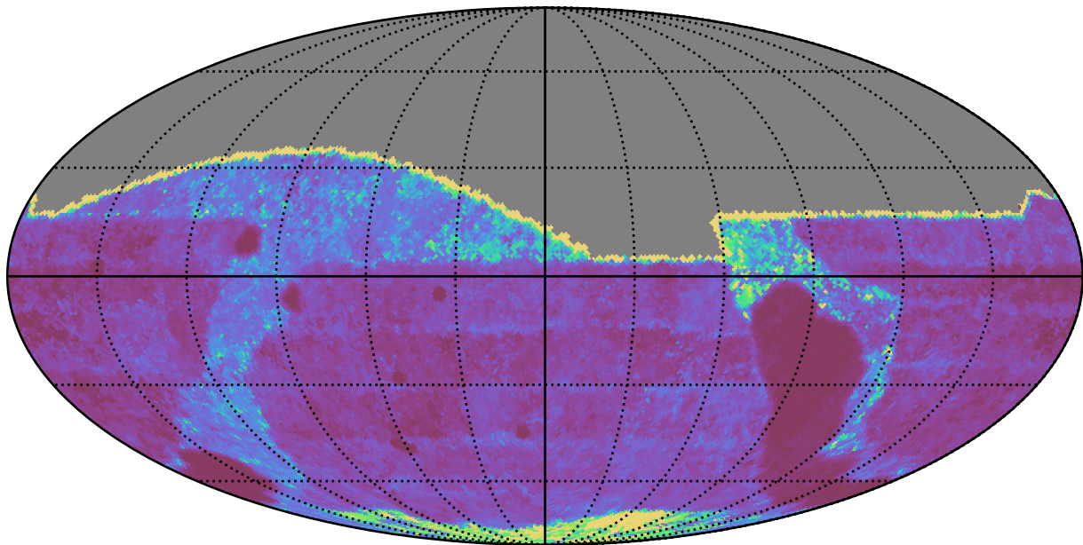
telescope_jerk_v3.5_10yrs All sky g band: Median Inter-Night Gap
