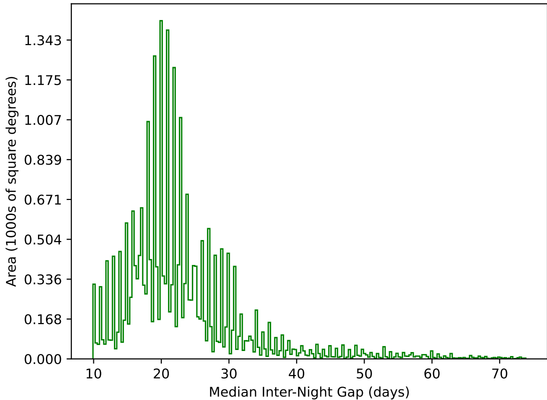
telescope_jerk_v3.5_10yrs All sky g band: Median Inter-Night Gap
