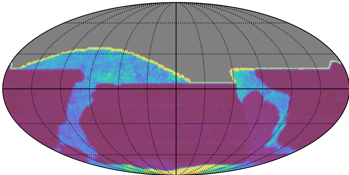
telescope_jerk_v3.5_10yrs All sky all bands: Median Inter-Night Gap
