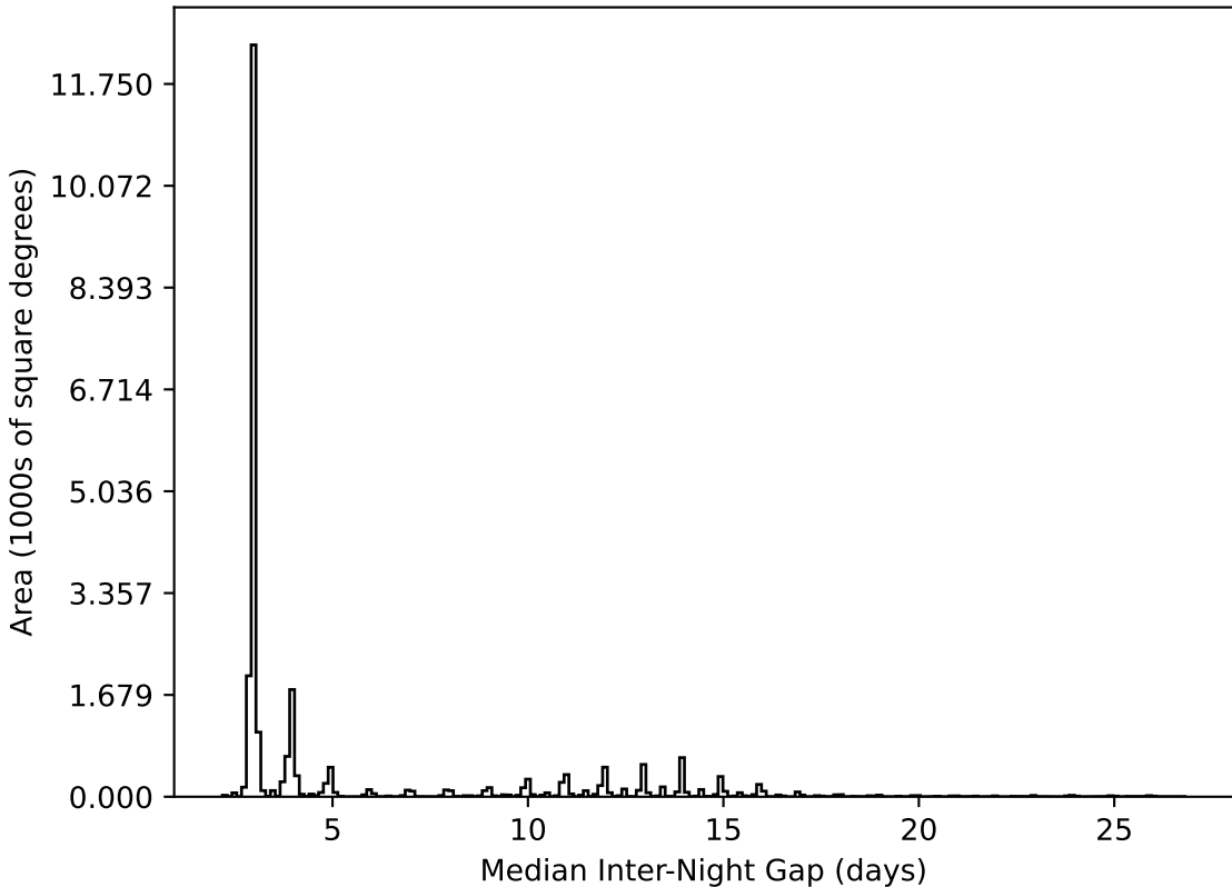
telescope_jerk_v3.5_10yrs All sky all bands: Median Inter-Night Gap
