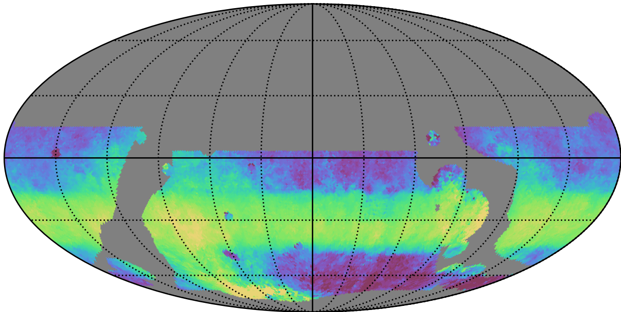
telescope_jerk_v3.5_10yrs WFD y band: Median HA
