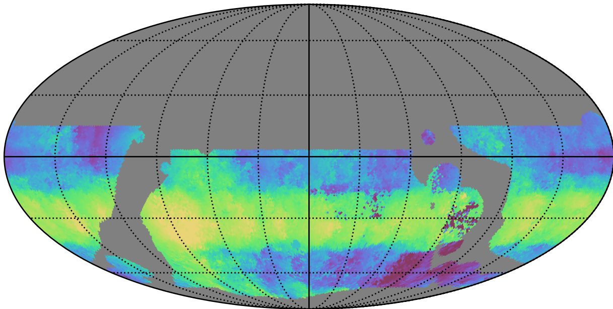
telescope_jerk_v3.5_10yrs WFD u band: Median HA
