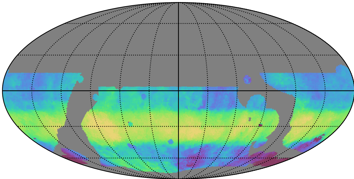
telescope_jerk_v3.5_10yrs WFD i band: Median HA
