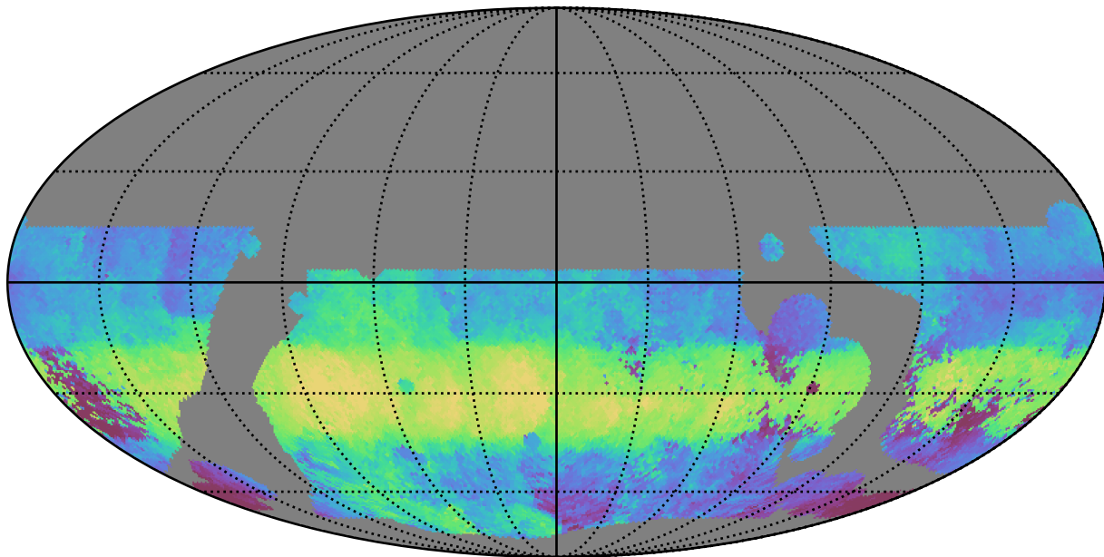
telescope_jerk_v3.5_10yrs WFD g band: Median HA
